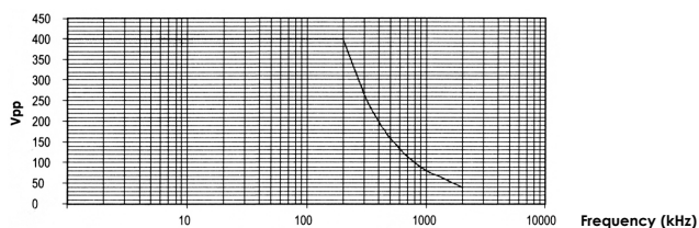
Figure 3: Maximum Vpp vs. Frequency Amplifier's maximum peak-to-peak output roll off with frequency. This is due to the amplifier's slew rate of 250 V/ \mu Sec.
